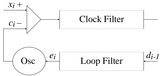
Figure 5. Phase-Lock Loop Model
