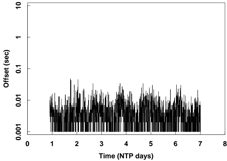
Figure 7. Filtered Offsets
