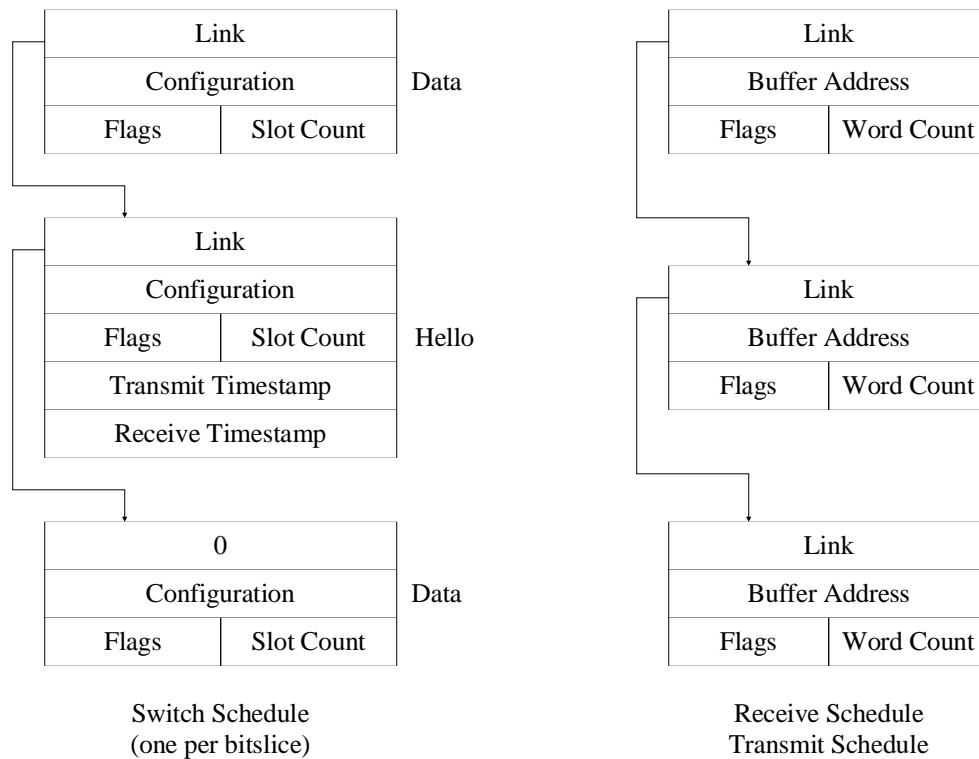
Figure 3. Burst Schedules
