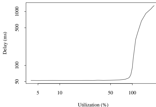
Figure 13. Utilization-Delay
