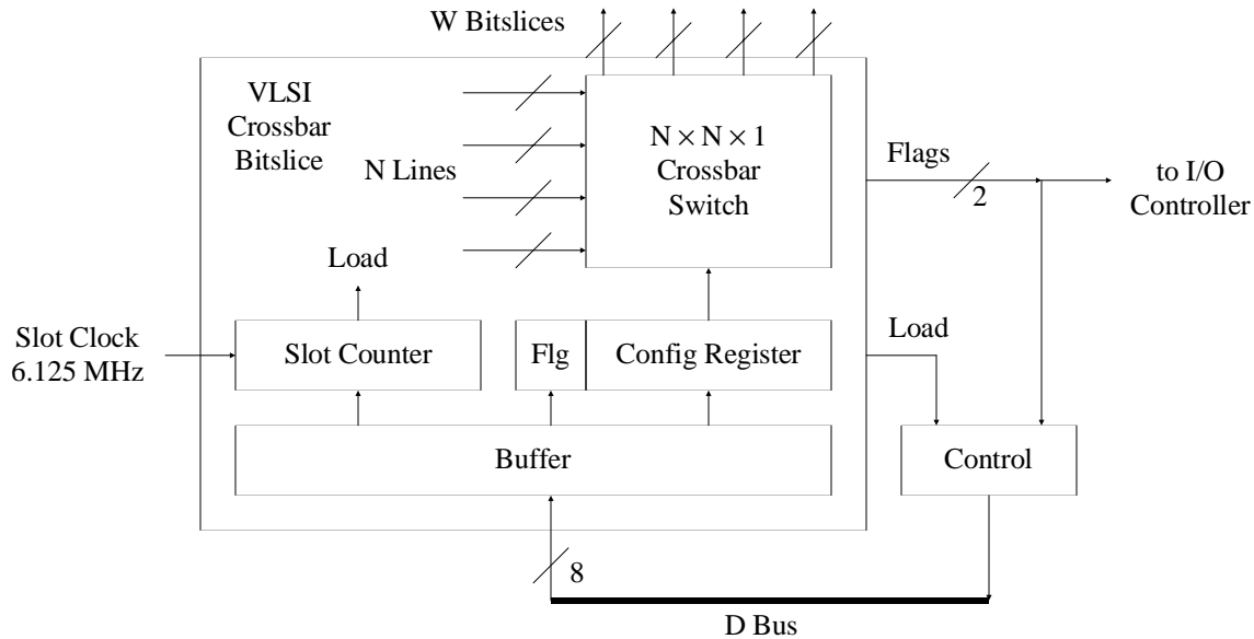
Figure 6. Switch Controller
