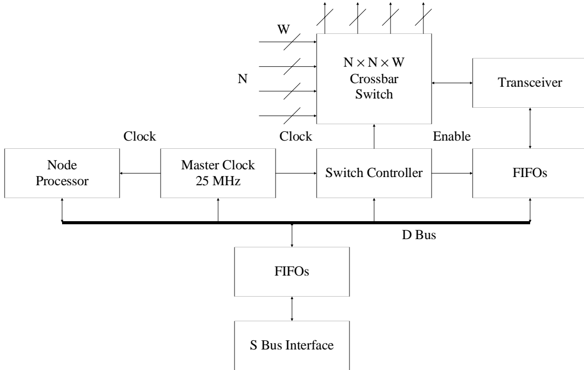
Figure 5. Node Controller
