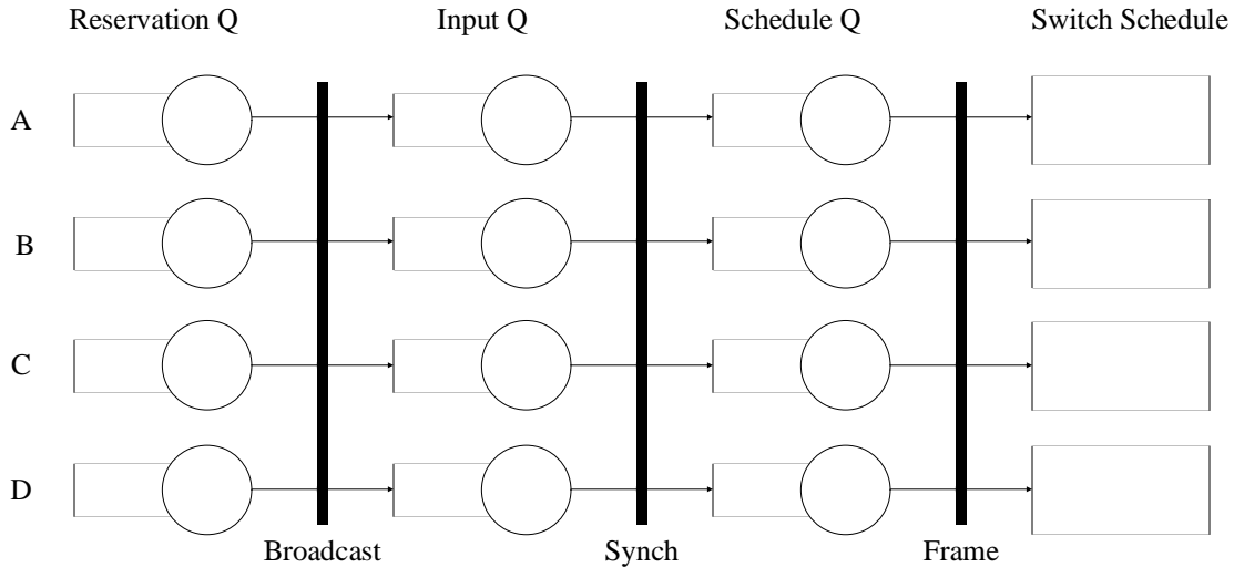
Figure 12. Software Queues
