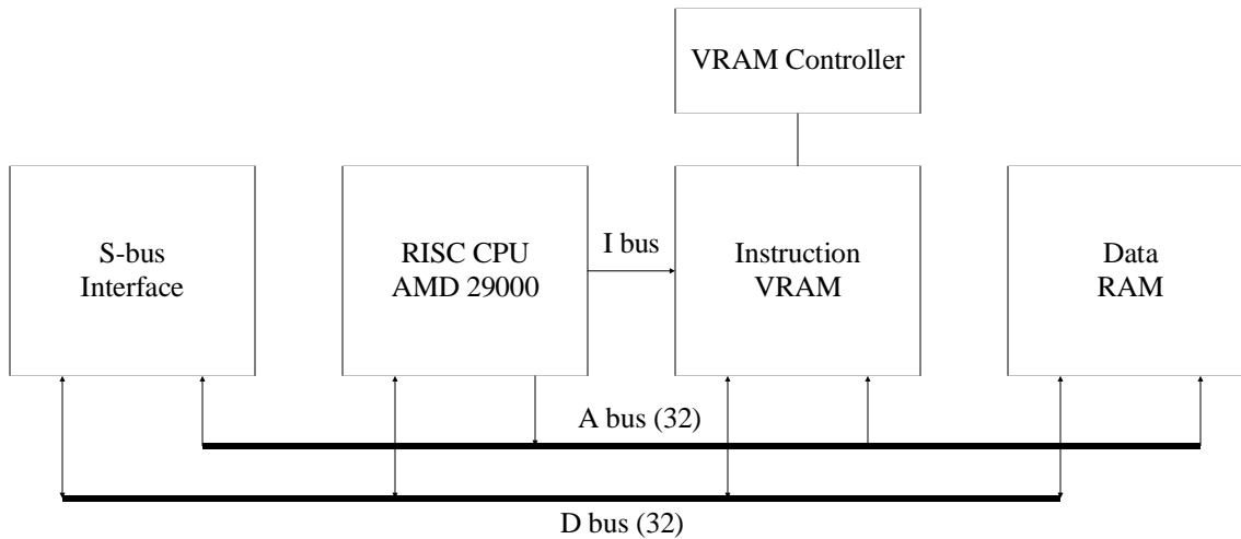
Figure 9. Node Processor
