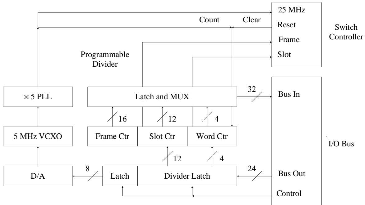
Figure 8. Master Clock
